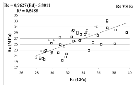
Figure 12. Correlation between compressive strength (Rc) and the dynamic elastic modulus (Ed).
