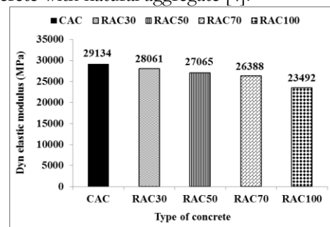
Figure 8. Elastic modulus as a fraction of concrete types at 28 days.
