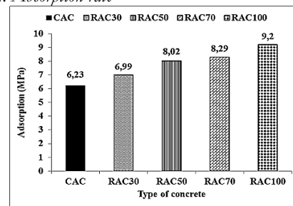
Figure 5. Absorption rate for the different types of concretes.
