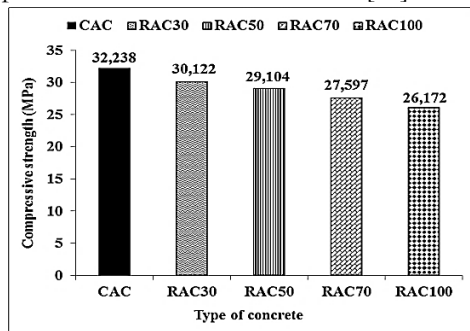
Figure 6. Compressive strength as a function of percentage of recycled aggregate replacement at 28 days.
