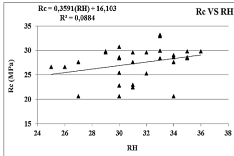
Figure 10. Correlation of compressive strength (Rc) and rebound hammer number (RH).
