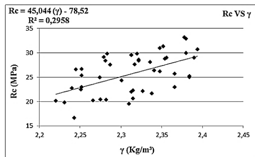
Figure 13. Correlation between the compressive strength and the density.
