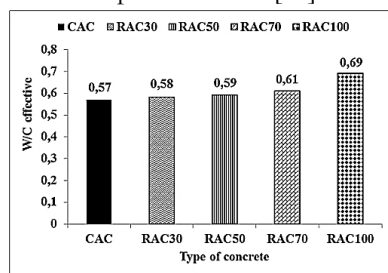
Figure 3. W/C ratio as a function of the percentage of replacement of recycled aggregate.
