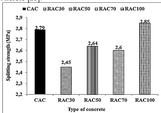
Figure 7. Tensile strength (Rt) for different types concretes at 28 days of age.
