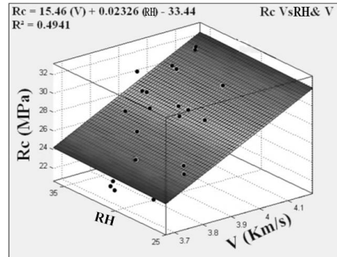
Figure 11. Correlation between compressive strength (Rc), ultrasonic velocity (V) and rebound hammer number (RH).
