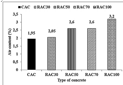
Figure 2. Air content for the different types of concrete.
