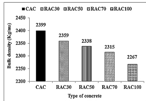
Figure 1. Density for the different concrete types.
