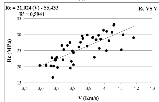
Figure 9. Correlation between compressive strength (Rc) and the ultrasonic velocity (V).
