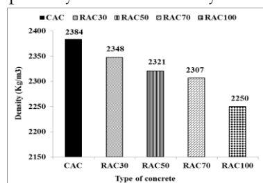
Figure 4. Density for the different types of concrete at 28 days of age.
